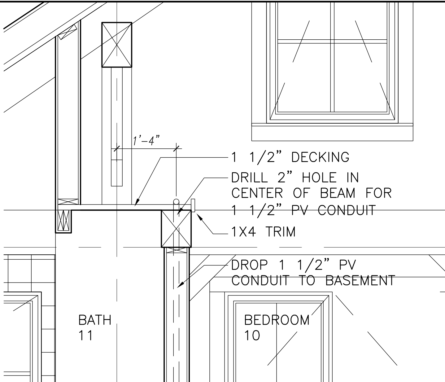
1 PARTIAL MONITOR PLAN 3/4" = 1'-0"
